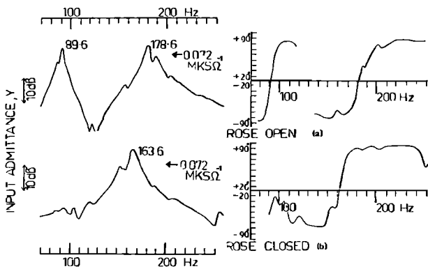
FIG. 5. Input admittance and its phase with respect to force of excitation measured at the center of the bridge with (a) the rose open and (b) the rose closed.
